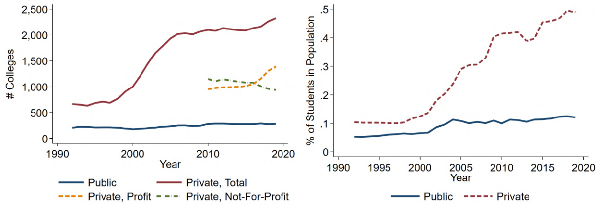
Figure A4: Evolution in the number of colleges and the share of college graduates in the population
