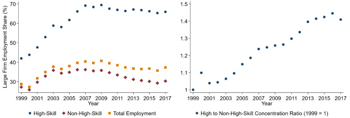
Figure 1: Evolution of high-skill concentration and the high to non-high-skill concentration ratio
