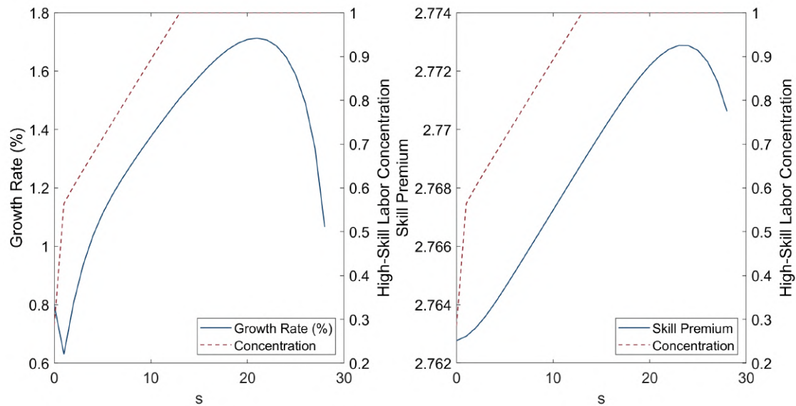
Figure A29: Growth rate, wage premium, and high-skill concentration as a function of the gap (without the non-innovative, outside firm)
