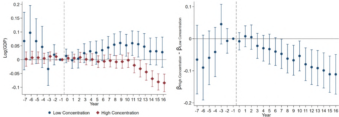
Figure A17: Difference-in-differences estimates of the effect of college creation on local growth at municipalities with high and low high-skill concentration (weighted by \log(\text{population}) )
