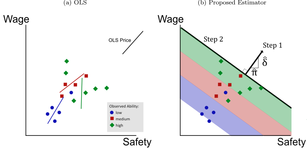
Figure 2: Graphical Intuition
