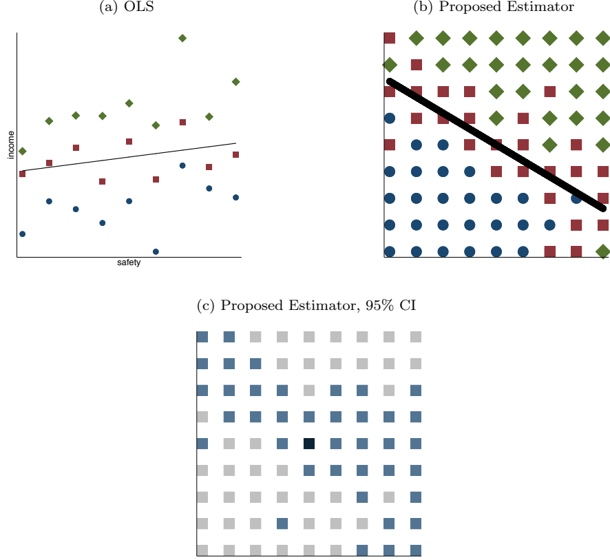
Figure 5: Non-Parametric & Linear
